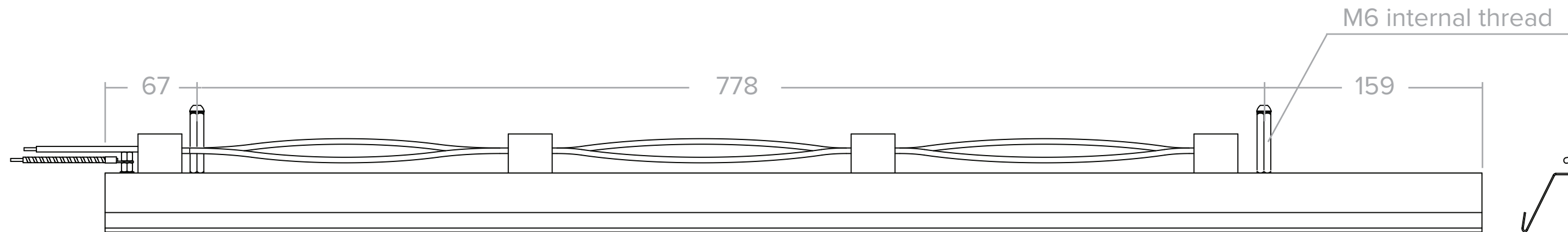
Side view
