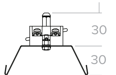
End view
