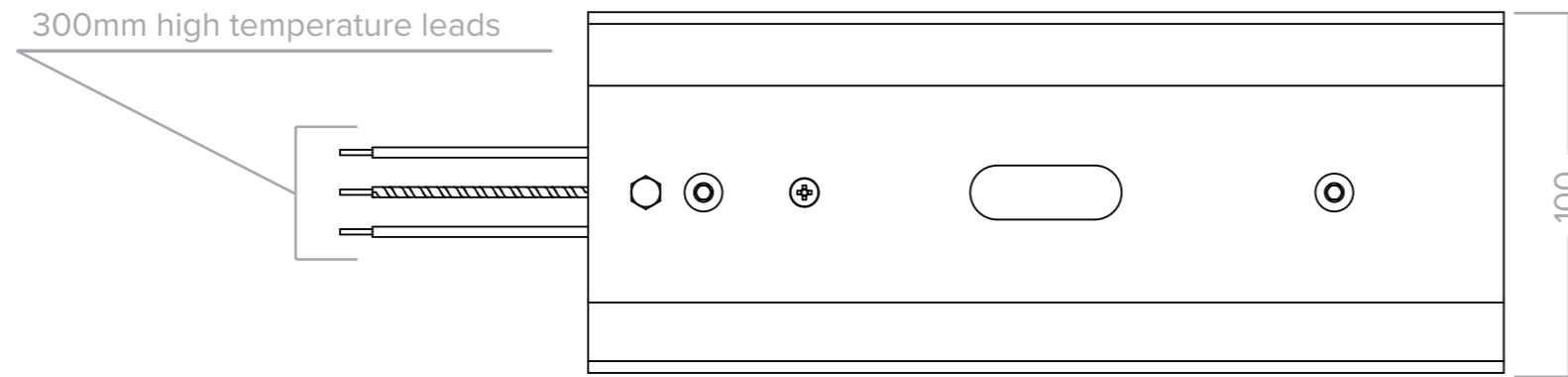
Front view
