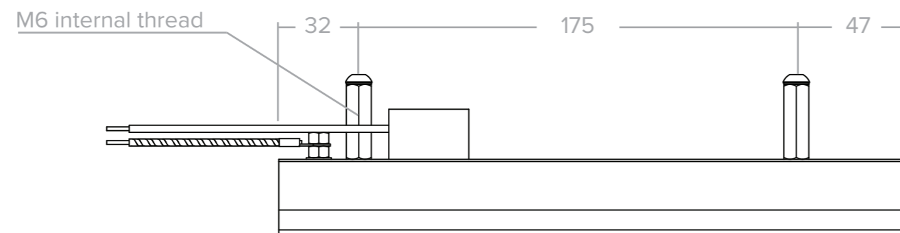
Side view
