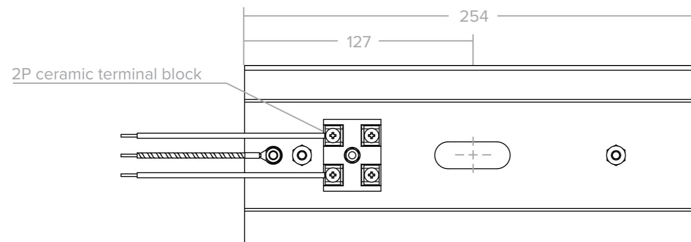
Rear view
