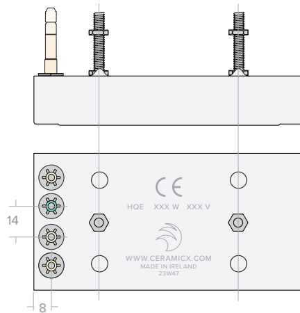
THERMOCOUPLE POSITION FOR HQE ELEMENTS HIGHER THAN 250W
