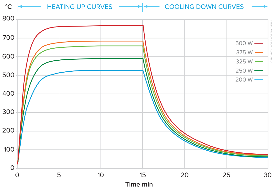
PHQE TcK Heat up and cool down curves showing average surface temperature measured with a thermal imaging camera set to an emissivity of 0.7
