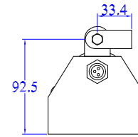
END VIEW - CONDUIT EXIT SIDE
