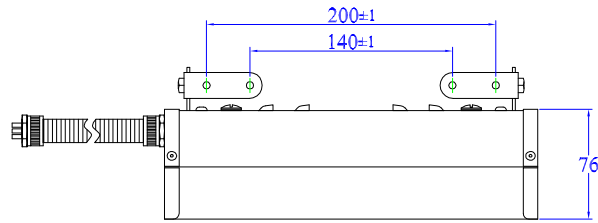
SIDE VIEW WITH MOUNTING BRACKETS ASSEMBLED
