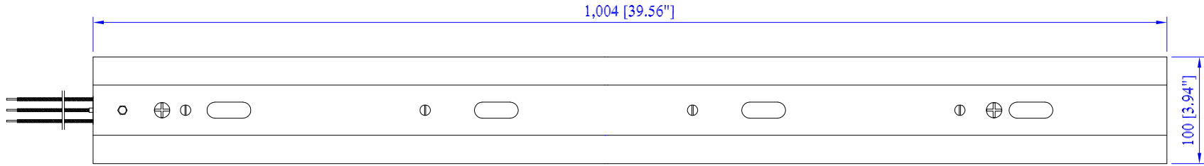
FRONT VIEW
