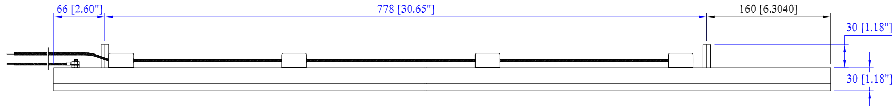
SIDE VIEW
