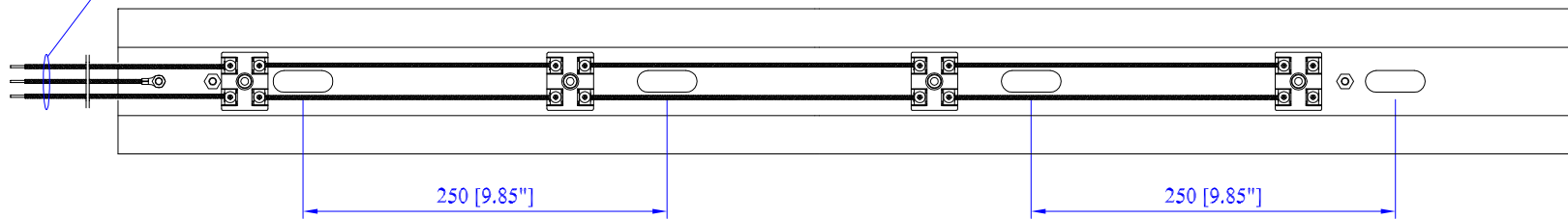
TOP VIEW
